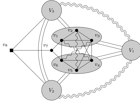
Figure 21: Schematic drawing of strips in \mathcal{Z}_{15} (Hex-expansions of sporadic exception #1). V_2 is strongly complete to V_3 , and the adjacency between (V_1, V_2) and (V_1, V_3) is arbitrary. The pairs v_1, v_4 and v_3, v_6 are semiadjacent, and the pair v_2, v_5 is either semiadjacent or strongly antiadjacent.
