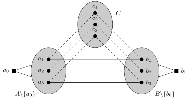
Figure 8: Schematic drawing of strips in \mathcal{Z}_2 (Near antiprismatic strips). The sets A, B, C are strong cliques. There is essentially a matching between the sets A \setminus \{a_0\} and B \setminus \{b_0\} , and there are essentially complements of matchings between the sets A \setminus \{a_0\} and C and between the sets B \setminus \{b_0\} and C .
