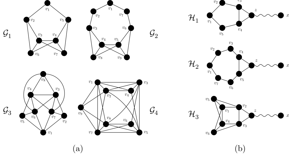
Figure 1: Forbidden induced subgraphs for fractionally co-strongly perfect graphs. (a) The graphs G_1, G_2, G_3, G_4 . (b) Hefts H that are combined to construct skipping ropes.
