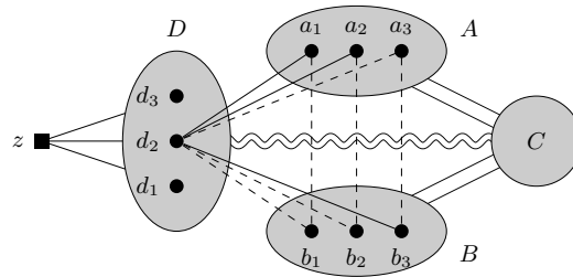
Figure 15: Schematic drawing of strips in \mathcal{Z}_9 (Special type of antiprismatic strips). There is essentially a complement of a matching between A and B . For every i and every d , d is strongly adjacent to one of a_i, b_i , and strongly antiadjacent to the other. The adjacency between C and D is arbitrary.
