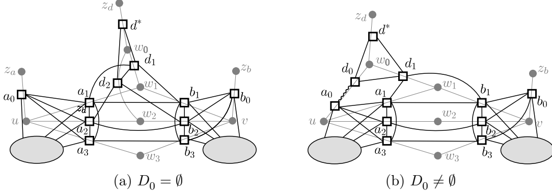
Figure 4: The construction of a larger strip-structure in (4.10). The gray vertices and edges represent the relevant submultigraph of H' . The black vertices and edges represent the relevant induced subtrigraph of T' . The gray ellipses represent the sets K_1 and K_2 . The ‘wiggly’ edge represents a semiedge. The black vertices are drawn on top of the gray edges to indicate to which strip each black vertex belongs.
